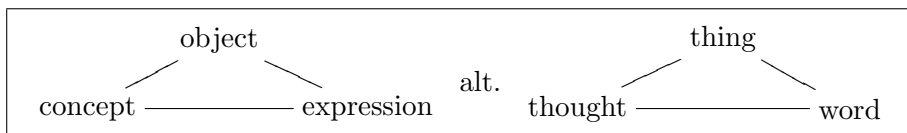
Figure 1. The relation between object, concept, and expression, as well as between thing, thought, and word.
