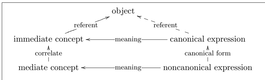
Figure 3. Mediate and immediate concepts compared with canonical and noncanonical expressions.
