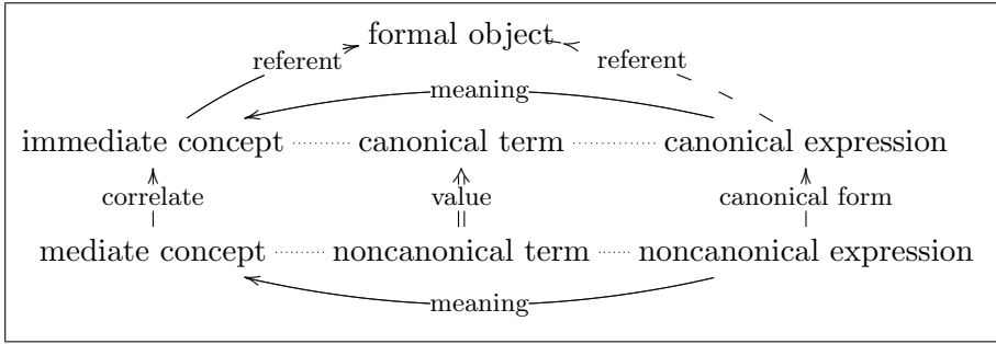
Figure 6. For beings of reason we get a threefold correspondence between expression, concept, and formal object.
