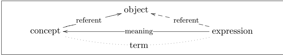
Figure 2. Meaning, referent, and term added to the triangle picturing the threefold correspondence between object, concept, and expression.
