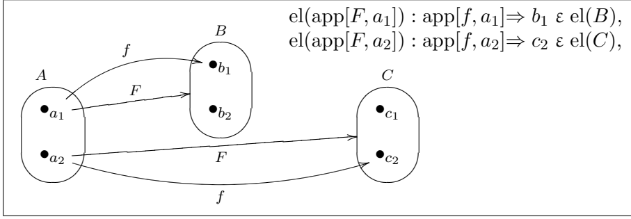
Figure 8. Diagram exemplifying a dependently typed function f on a set A with two elements a_1 and a_2 ; f takes a_1 to b_1 and a_2 to c_2 .
