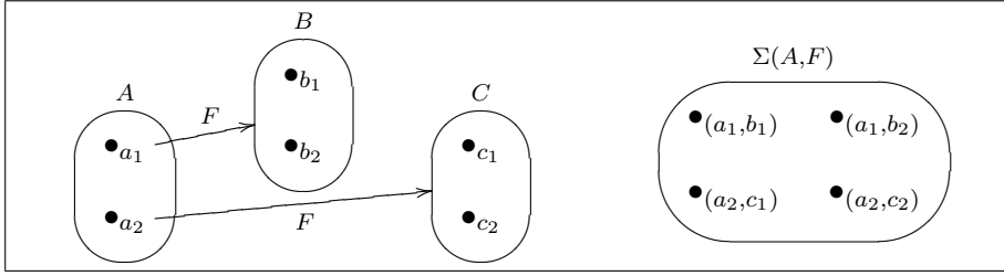
Figure 7. The disjoint union \Sigma(A, F) of a family F of sets over a set A with two elements a_1 and a_2 which takes a_1 to the set B = \{b_1, b_2\} and a_2 to the set C = \{c_1, c_2\} .
