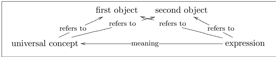
Figure 5. The threefold correspondence for universal concepts, which refer to many objects. In this figure there are two objects, but there can be arbitrarily many.
